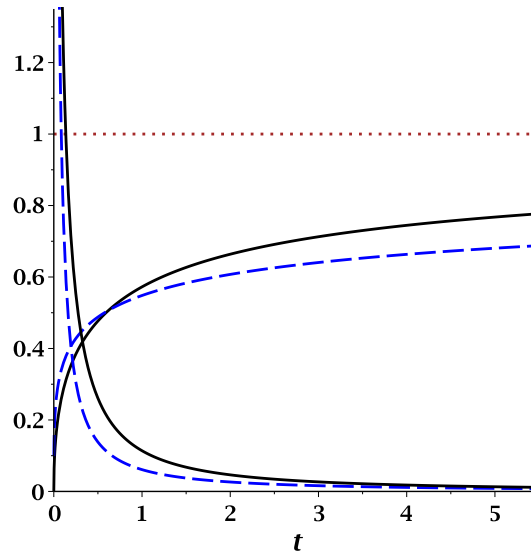
Figure 1: Solutions (1.5), (1.6), (4.15) and (4.21).
