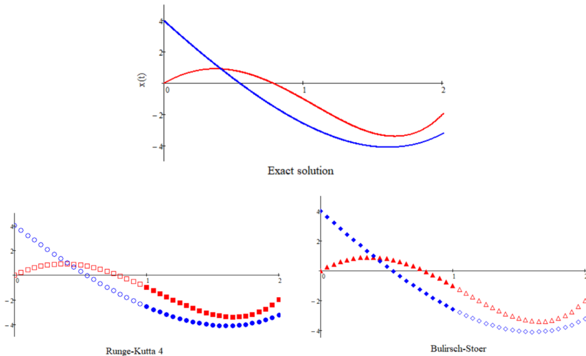
Figure 2: At h=0.05 in Problem D
