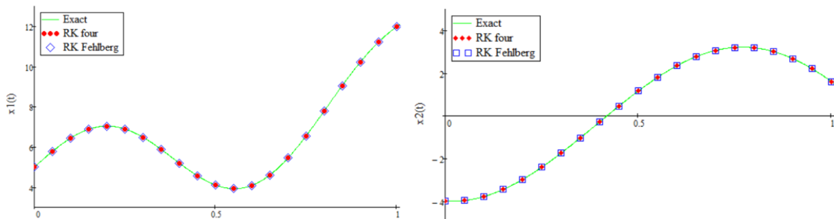
Figure 3: The exact solution and the numerical solutions of (46), (47)
