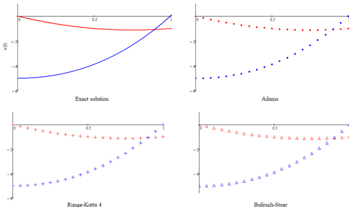
Figure 1: At h=0.05 in Problem A
